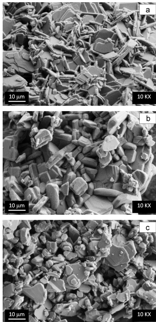
Fig. 6. Morphologies of the BIT powders prepared at (a) pH 3, (b) pH 5 and (c) pH 7.
