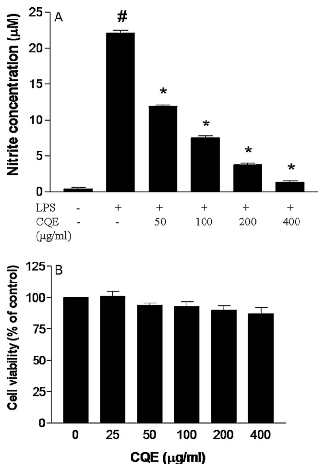
Fig. 1. Inhibition of nitrite production by CQE in LPS-stimulated RAW 264.7 macrophages. (A) Cells were co-incubated with the indicated concentrations of CQE (50–400 µg/ml) and LPS (1 µg/ml) for 24 h. The culture supernatants were subsequently isolated and analyzed for nitrite production. Each column shows the mean ± SD of three independent experiments with triplicate samples. # P < 0.001 vs. control and * P < 0.001 vs. LPS alone. (B) Viability of cells harvested at 24 h after the treatment with CQE (25, 50, 100, 200 and 400 µg/ml) was determined using the MTT test as described in Section 2. Each column shows the mean ± SD of three independent experiments with triplicate samples.
