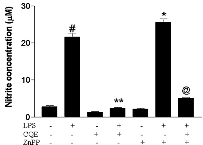
Fig. 6. HO-1 mediates the suppression of LPS-induced NO production in RAW 264.7 cells treated with CQE. Cells were pre-incubated with 10 µM ZnPP for 1 h before exposure to 400 µg/ml CQE and LPS (1 µg/ml) for 24 h. Each column shows the mean ± SD of three independent experiments with triplicate samples. # P < 0.001 vs. control, * P < 0.01 and ** P < 0.001 vs. LPS alone and @ P < 0.001 vs. LPS + CQE.
