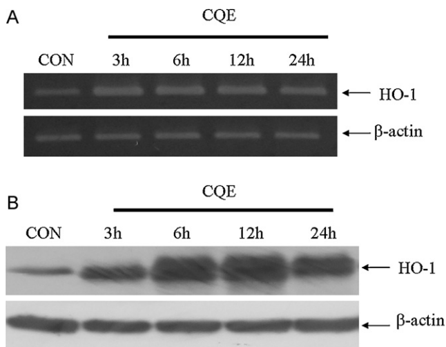
Fig. 5. Induction by CQE of HO-1 protein expression in RAW 264.7 cells. Cells were treated with 400 µg/ml CQE for 3, 6, 12 and 24 h. (A) Levels of HO-1 mRNA were determined by RT-PCR analysis. (B) Levels of HO-1 protein were determined by Western blotting analysis. β-Actin expression was used as an internal control. CON, cells without any treatment.
