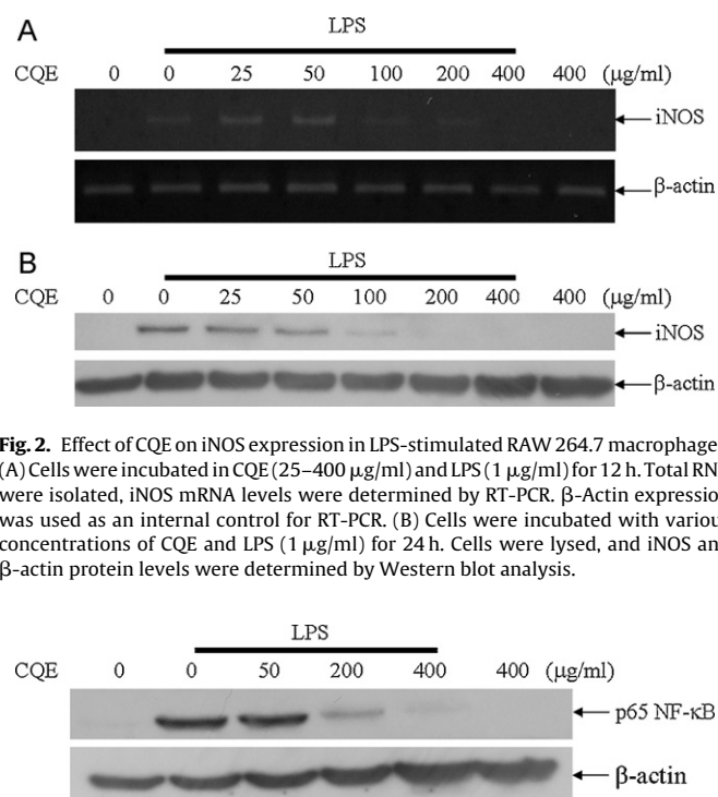
Fig. 3. Effects of CQE on the p65 NF-κB nuclear translocation. RAW 264.7 cells were co-incubated with CQE (50, 200 and 400 µg/ml) and LPS (1 µg/ml) for 2 h. The levels of p65 subunit in nuclear protein were determined by Western blotting analysis.
